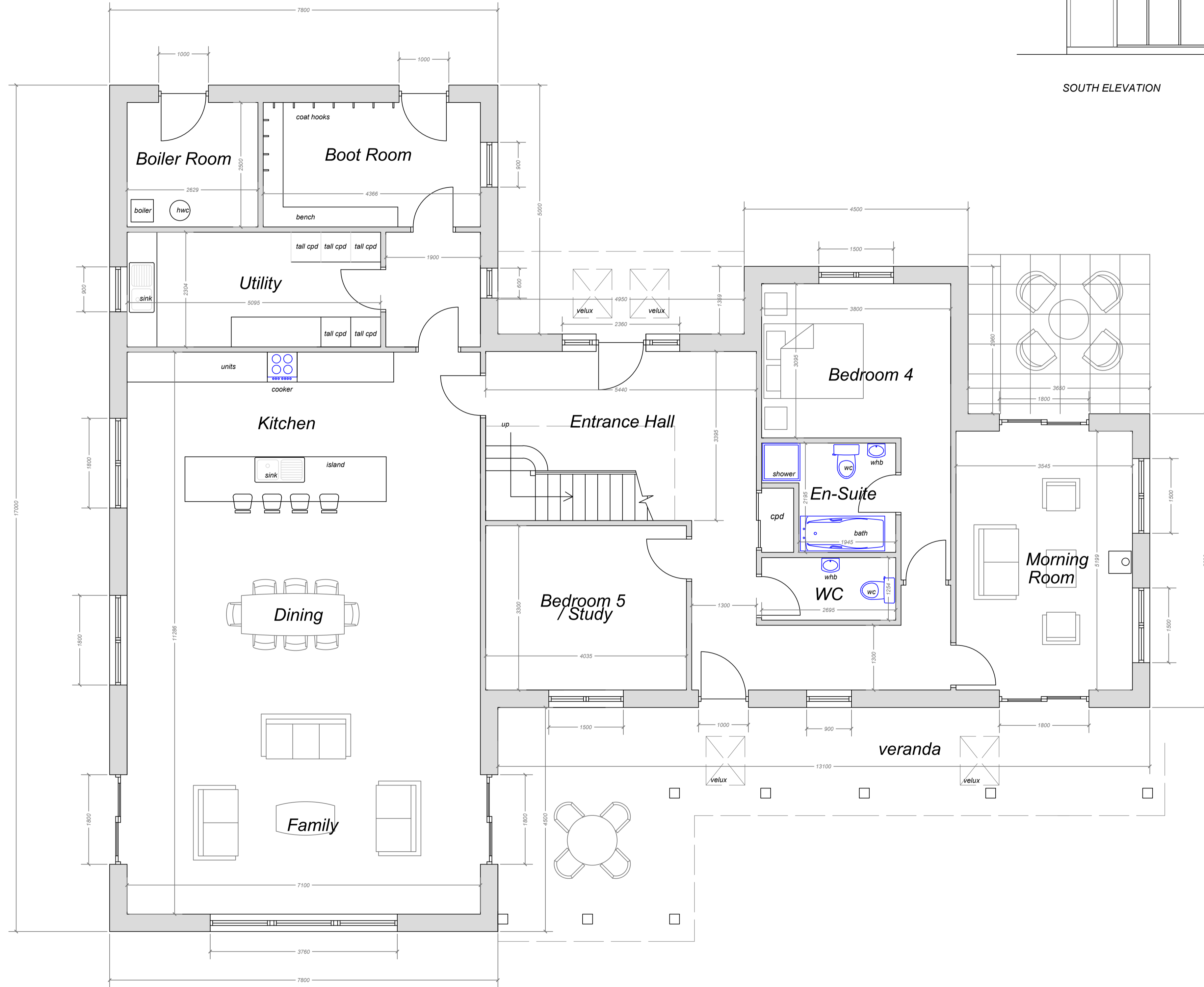
GROUND FLOOR PLAN (204m 2 )
